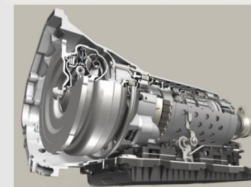
ZF-AS Tronic
